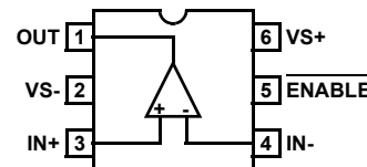
EL8188 (6-PIN SOT-23) TOP VIEW
