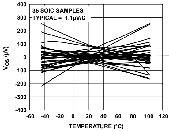
FIGURE 13. SOIC V_{OS} vs TEMPERATURE ( V_S = 5V )
